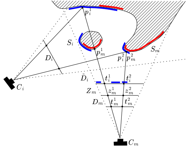
Fig. 6. Occlusions example: point p_i^1 is visible from camera position C_i , but not from C_m . Since the detail map D_i is projected onto the image plane of D_m , this point must be discarded. The depth map Z_m corresponding to scan S_m is used to mask points of S_i which are not visible from C_m . In contrast, point p_i^2 is visible from C_m and its texture is recorded onto \tilde{D}_i . The red and blue curves identify the two scans S_m and S_i , respectively. The areas of \tilde{D}_i that receive texture from scan S_i are also highlighted in blue.
