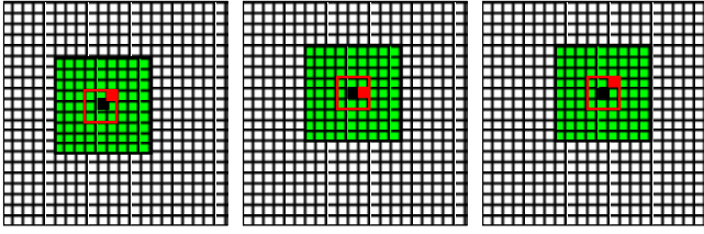
Fig. 7. Sliding-window search for the point maximizing cross-correlation between image neighborhoods. The search starts at point t_i \in \tilde{D}_i , marked in black. The green area is cross-correlated to the corresponding area in D_m . The operation is repeated for areas centered in all pixels within the search region outlined in red. The pixel corresponding to the center of the maximum cross-correlation area is marked in red. The search window is moved to the new center and a new iteration starts.
